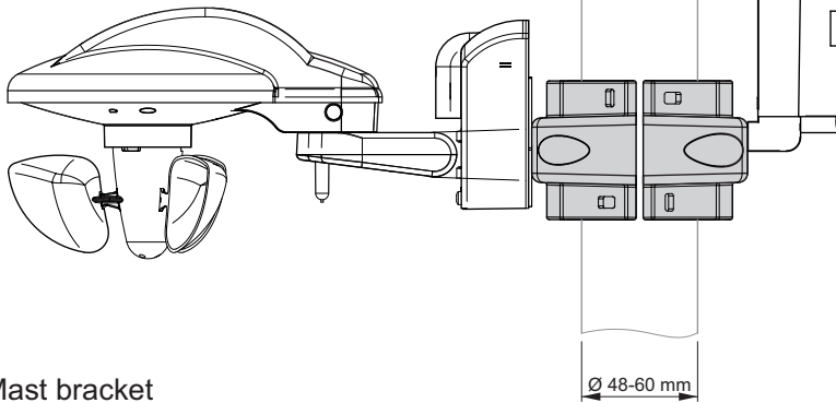
Mast bracket
