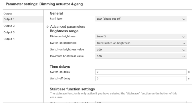
Advanced parameter settings for the dimming actuator
