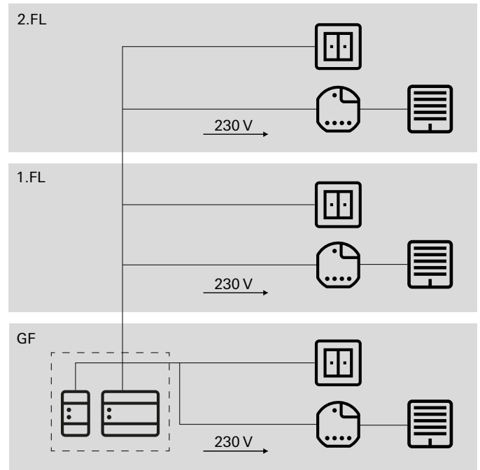
Centralised actuator installation
