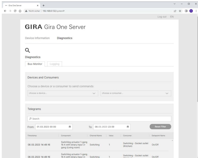
Diagnostic monitor
